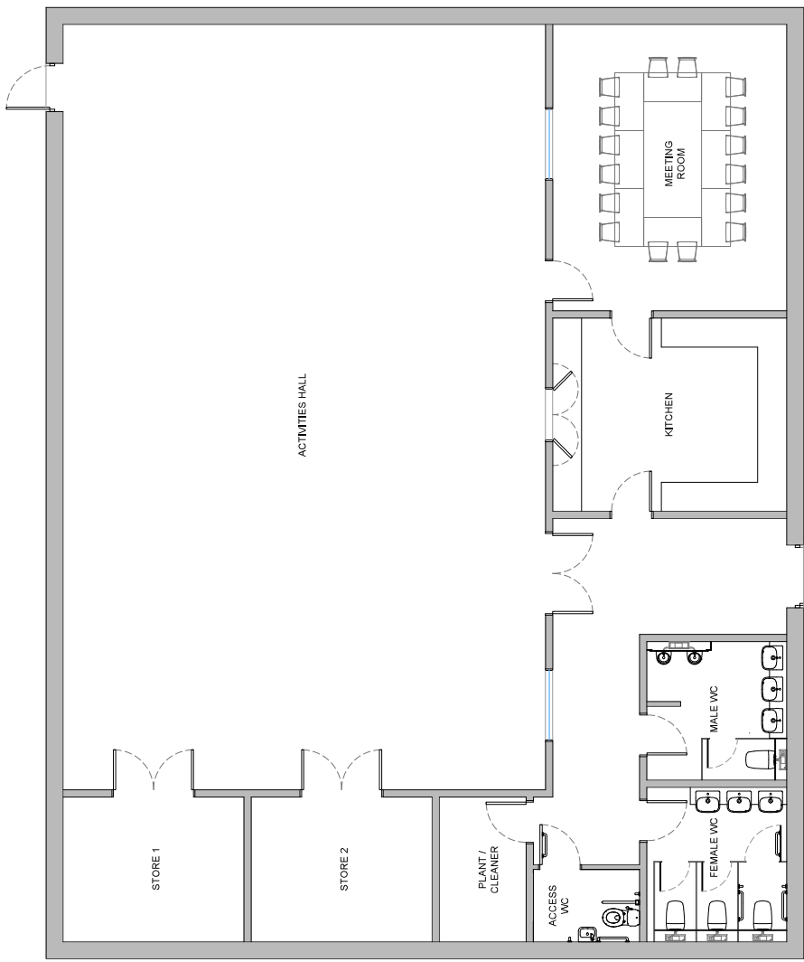
PROPOSED FLOOR PLAN Scale 1:50
